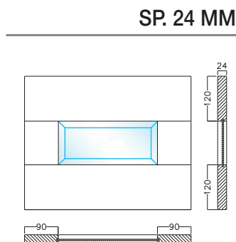
cestone vetro frassino bianco assoluto (opz.2460M) absolute white ash glass deep drawer (code 2460M)
