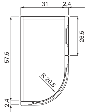
BASE TERMINALE stondata con anta open END BASE UNIT with curved door
