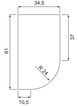
TOP PER BASE TERMINALE stondata con anta WORKTOP FOR END BASE UNIT open with curved door
